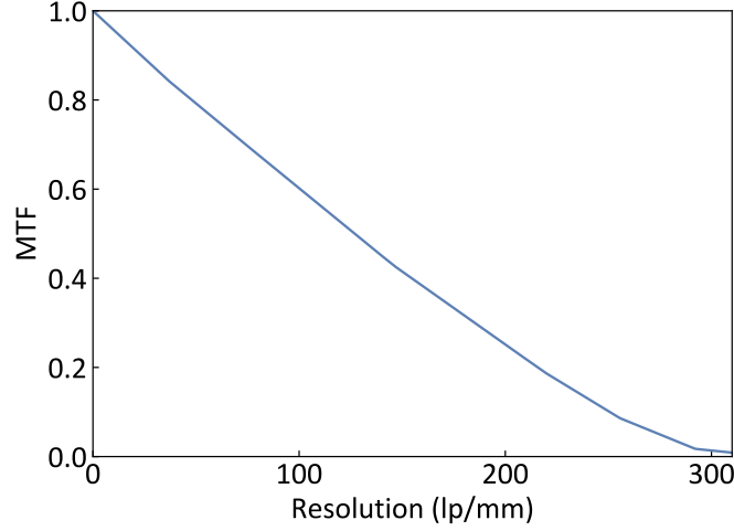
Figure 5.9: MTF of the vertical imaging objective. The curve shows how the contrast is going down with increasing resolution. The cut-off frequency is at 310.45 lp/mm.
